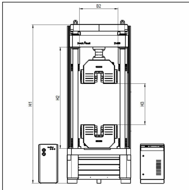
Drawing: Z1600E with hydraulic grips
